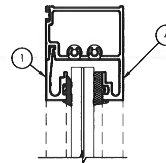
2 VERTICAL CROSS SECTION 4
