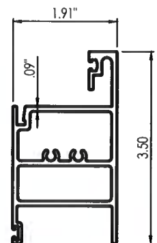
58 BOTTOM RAIL - FIXED PANEL 9/16" GLASS
