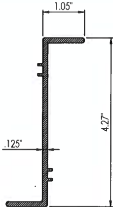
13 OXO REINFORCEMENT
