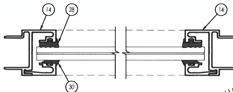
3 HORIZONTAL CROSS SECTION 4
