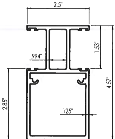
15 XX ADAPTOR
