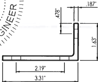
43 TOE ANCHOR
