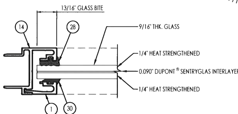
G2 GLAZING DETAIL MONOLITHIC 9/16" LAMINATED GLASS
