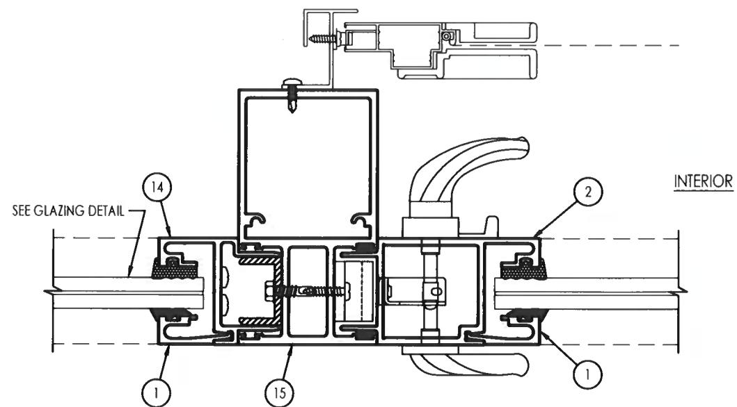
3 HORIZONTAL CROSS SECTION 7
