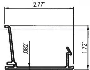
17 FRAME HEAD POCKET COVER
