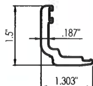
42 REACTION CLIP
